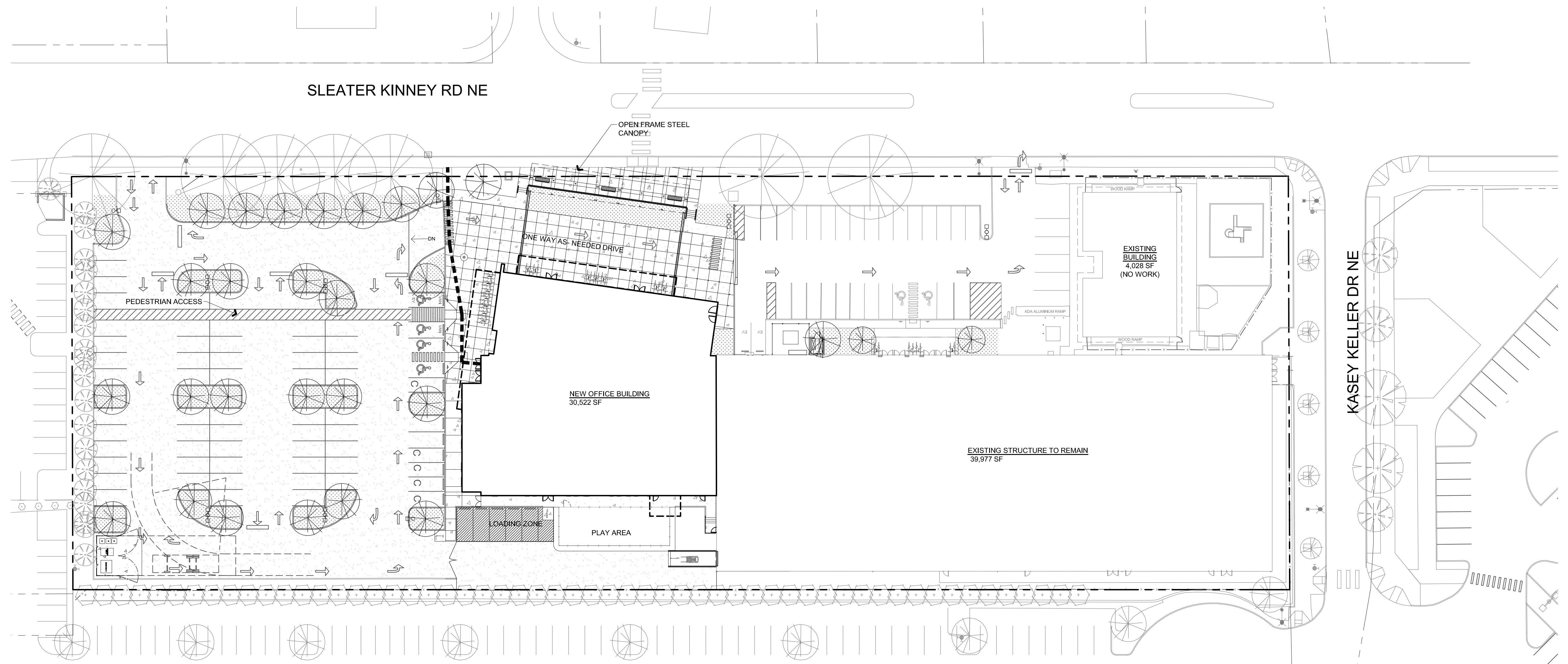
1 OVERALL SITE PLAN 1" = 30'
